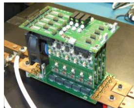
Multiphase 25-cell GaN interleaved converter (Vin=12-48V Vout=1-12V, 5x75A, Fsw =0.5-3MHz)
