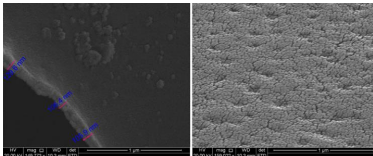
Cross section (left) and top view (right) of a chitosan membrane coated with honeybee wax.
